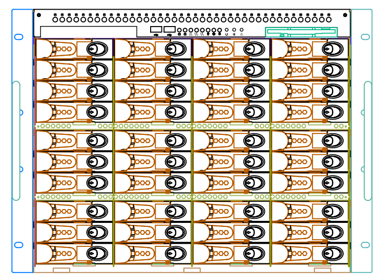
1 x Slim CD-ROM + 1 x Slim FDD 40 x 3.5" Hot Swap S-ATA HDD Front In-Side View
