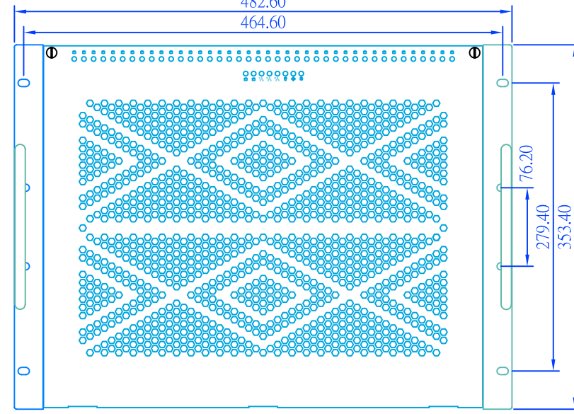
Front Out-Side View
