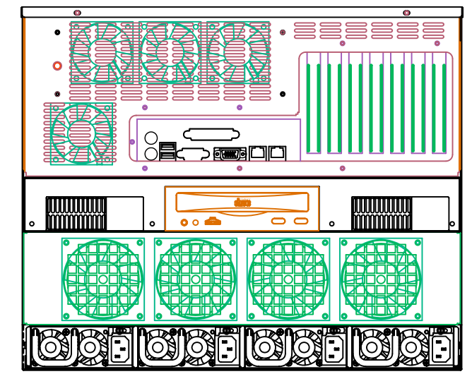
1 x 5.25" CD-ROM + 2 x 3.5" Hidden HDD 2 x 90 mm Blower (30.5CFM each) Rear View - 2
