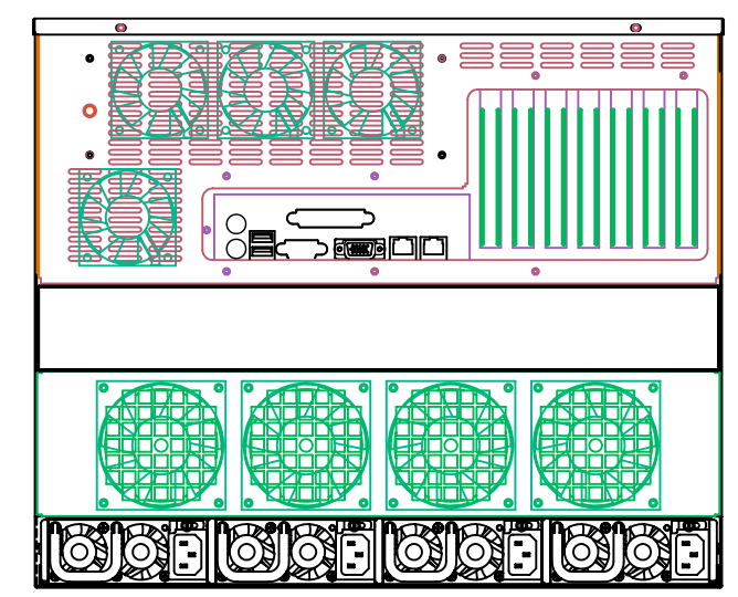
4 x 60 mm Fans (23.5 CFM ea.) 4 x 80 mm Fans (42.5 CFM ea.) Rear View - 1 (Standard)
